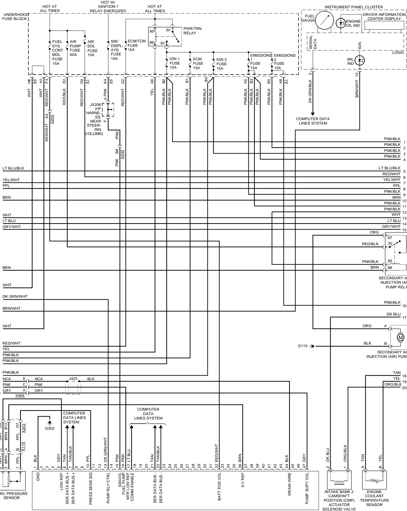
FUEL PUMP FLOW CONTROL MODULE
